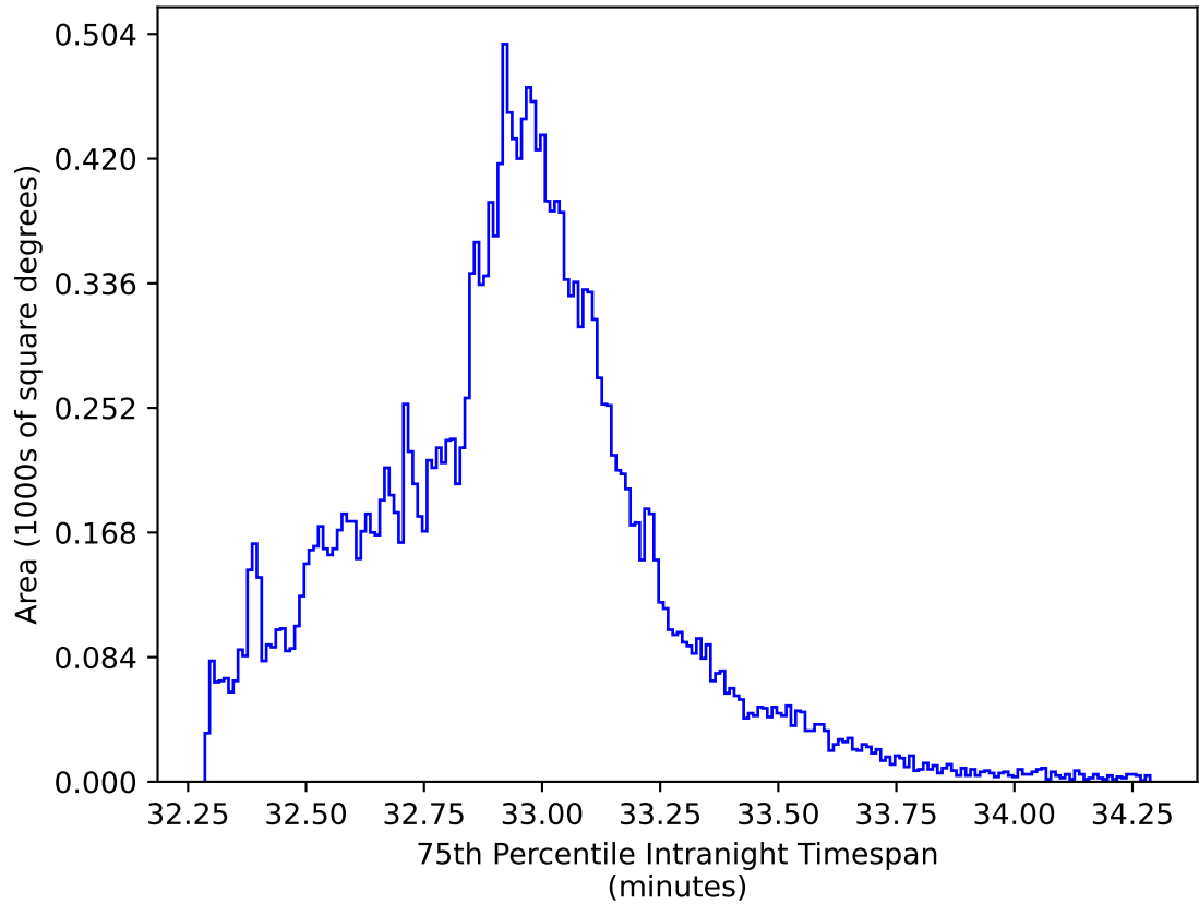
too_elab_r8_d3_giz_v3.4_10yrs All sky y band: 75th Percentile Intranight Timespan
