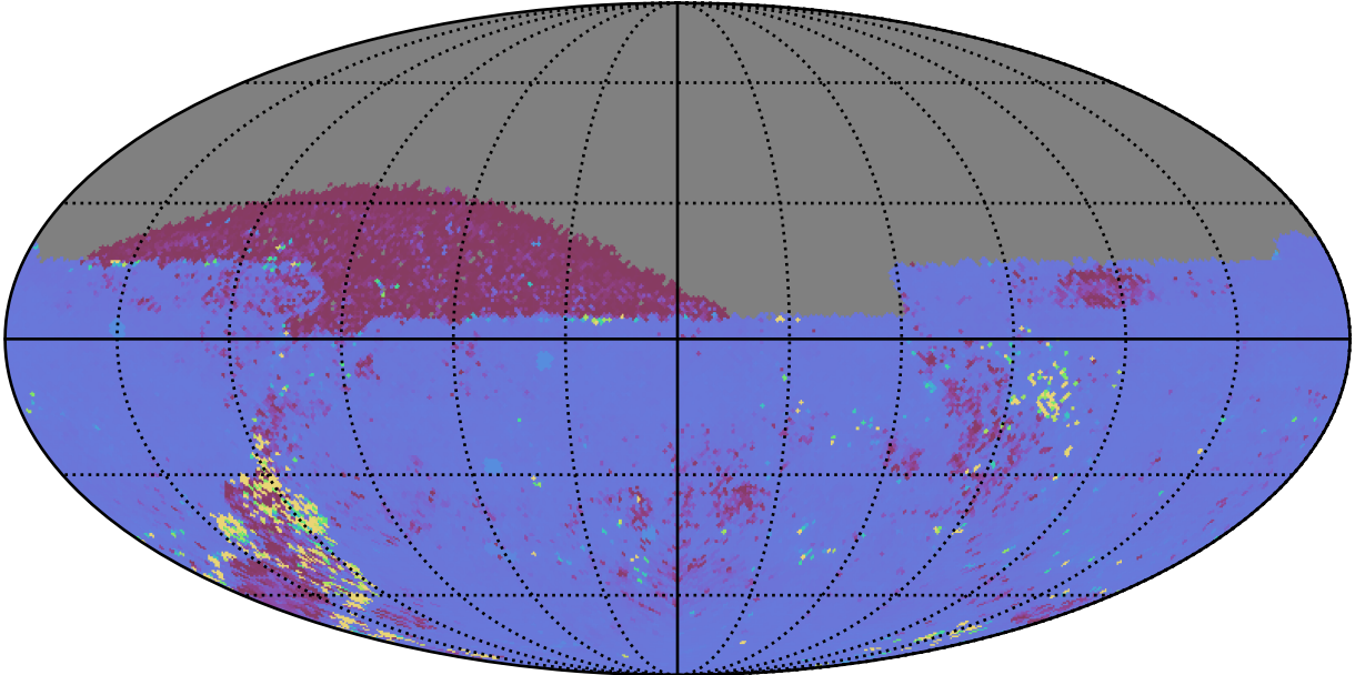
too_elab_r8_d3_giz_v3.4_10yrs All sky ug bands: 75th Percentile Intranight Timespan
