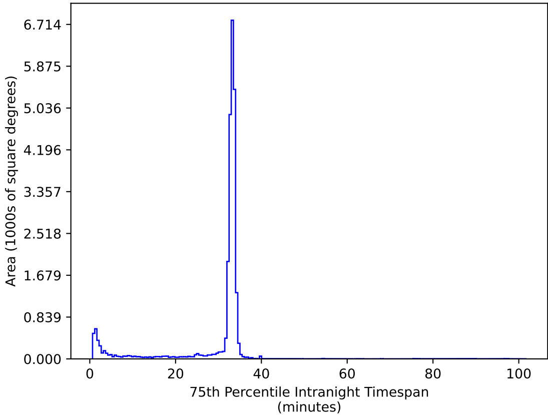
too_elab_r8_d3_giz_v3.4_10yrs All sky ug bands: 75th Percentile Intranight Timespan
