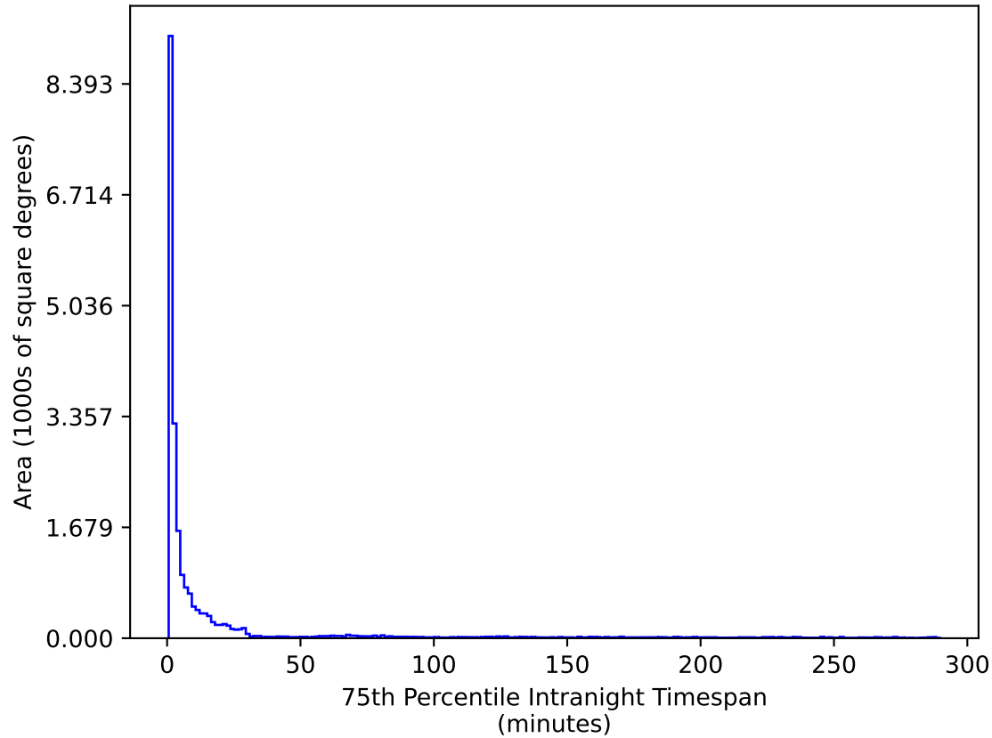
too_elab_r8_d3_giz_v3.4_10yrs All sky u band: 75th Percentile Intranight Timespan
