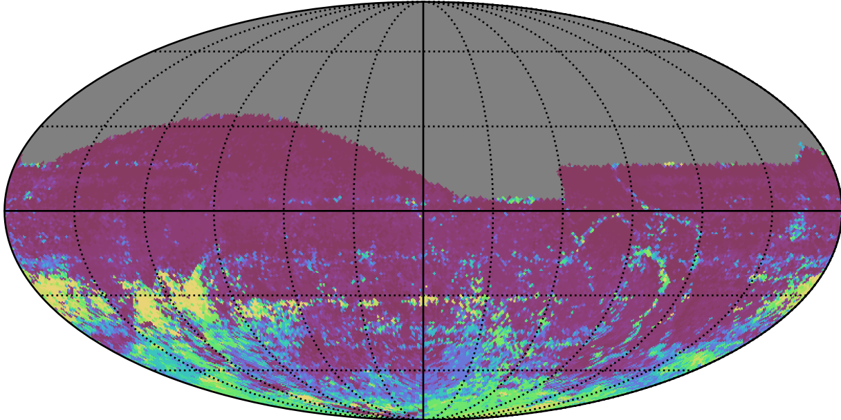
too_elab_r8_d3_giz_v3.4_10yrs All sky r band: 75th Percentile Intranight Timespan
