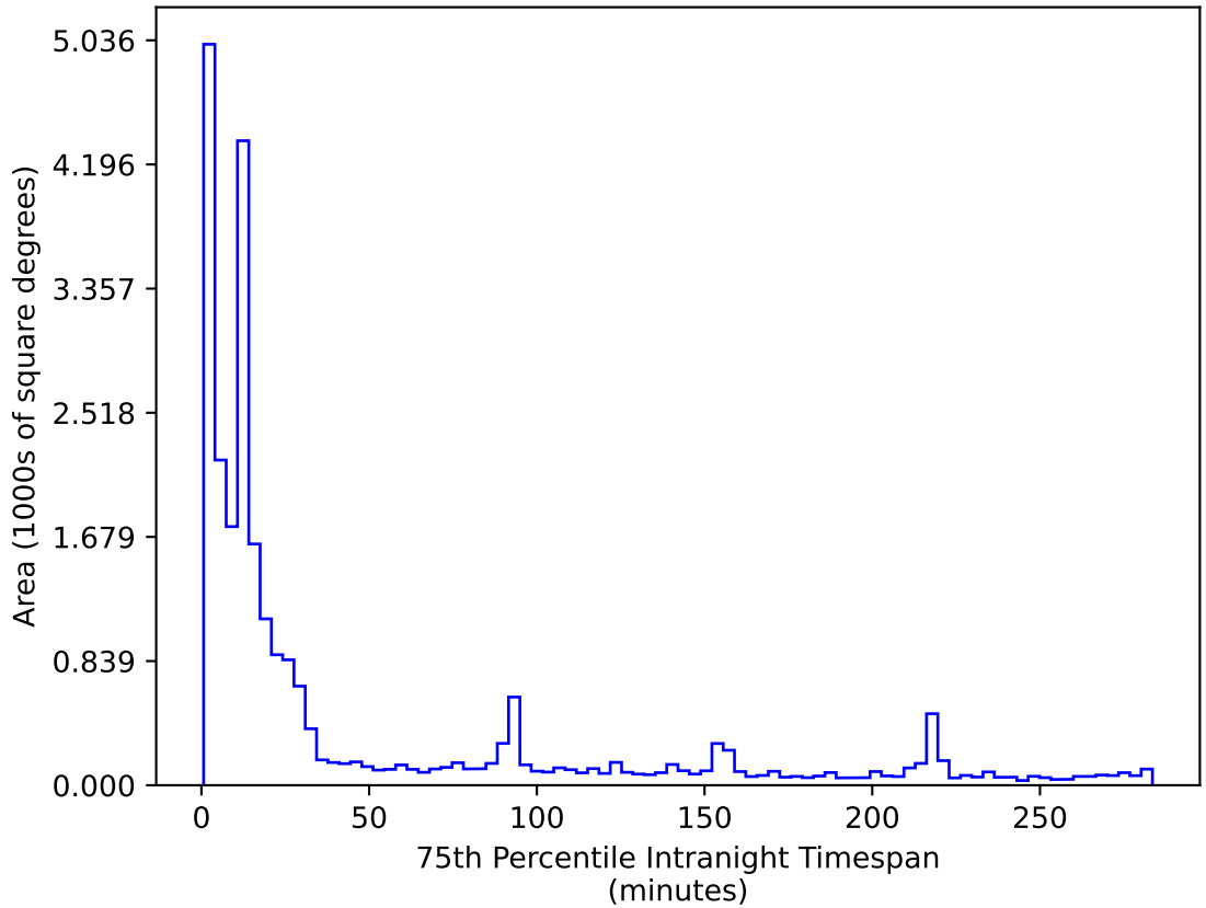
too_elab_r8_d3_giz_v3.4_10yrs All sky r band: 75th Percentile Intranight Timespan
