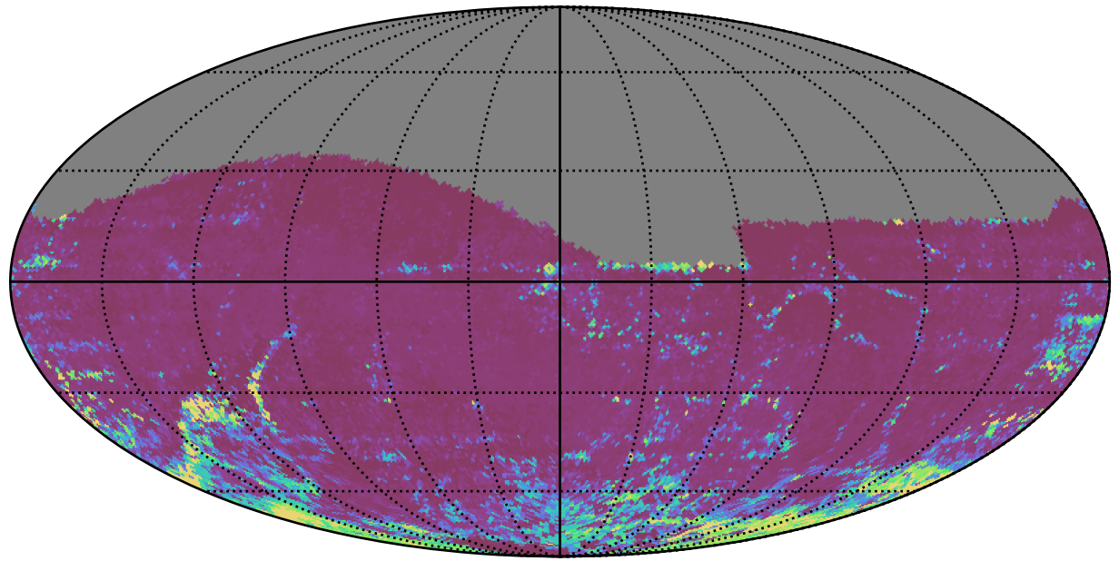
too_elab_r8_d3_giz_v3.4_10yrs All sky i band: 75th Percentile Intranight Timespan
