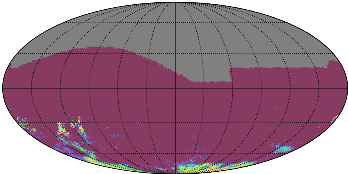
too_elab_r8_d3_giz_v3.4_10yrs All sky gr bands: 75th Percentile Intranight Timespan
