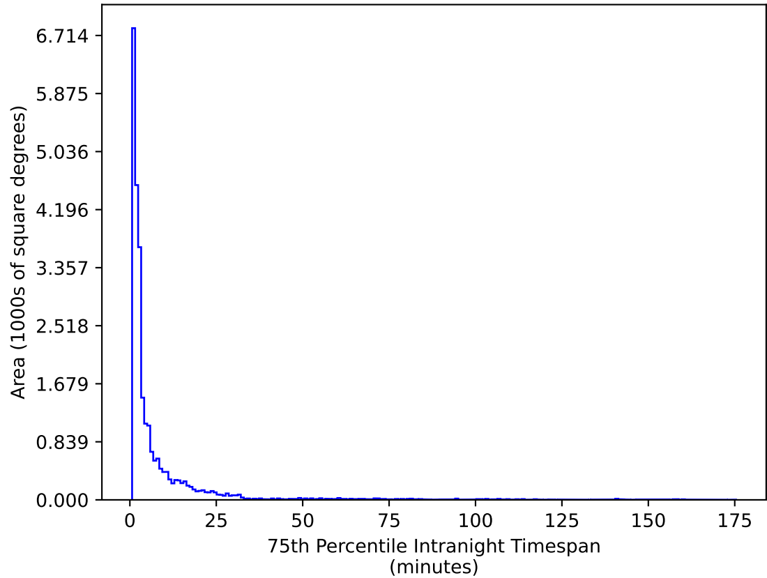
too_elab_r8_d3_giz_v3.4_10yrs All sky g band: 75th Percentile Intranight Timespan
