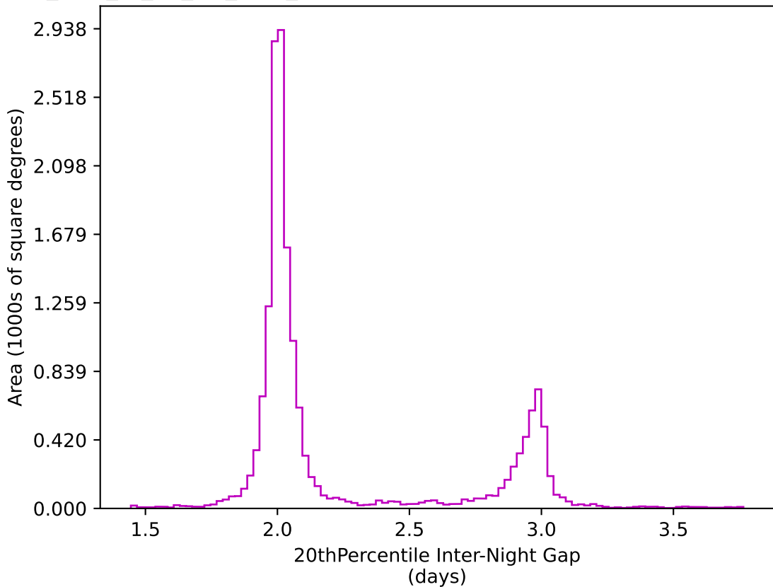
too_elab_r8_d3_giz_v3.4_10yrs WFD z band: 20thPercentile Inter-Night Gap
