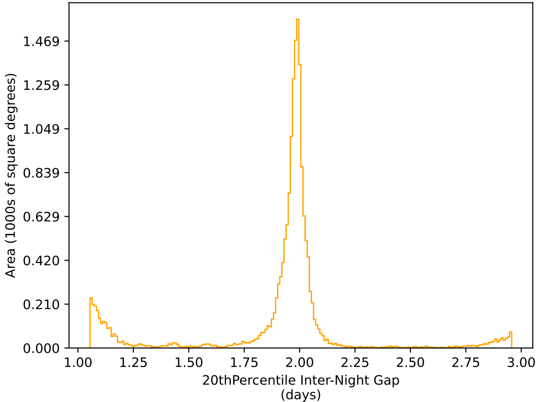
too_elab_r8_d3_giz_v3.4_10yrs WFD r band: 20thPercentile Inter-Night Gap
