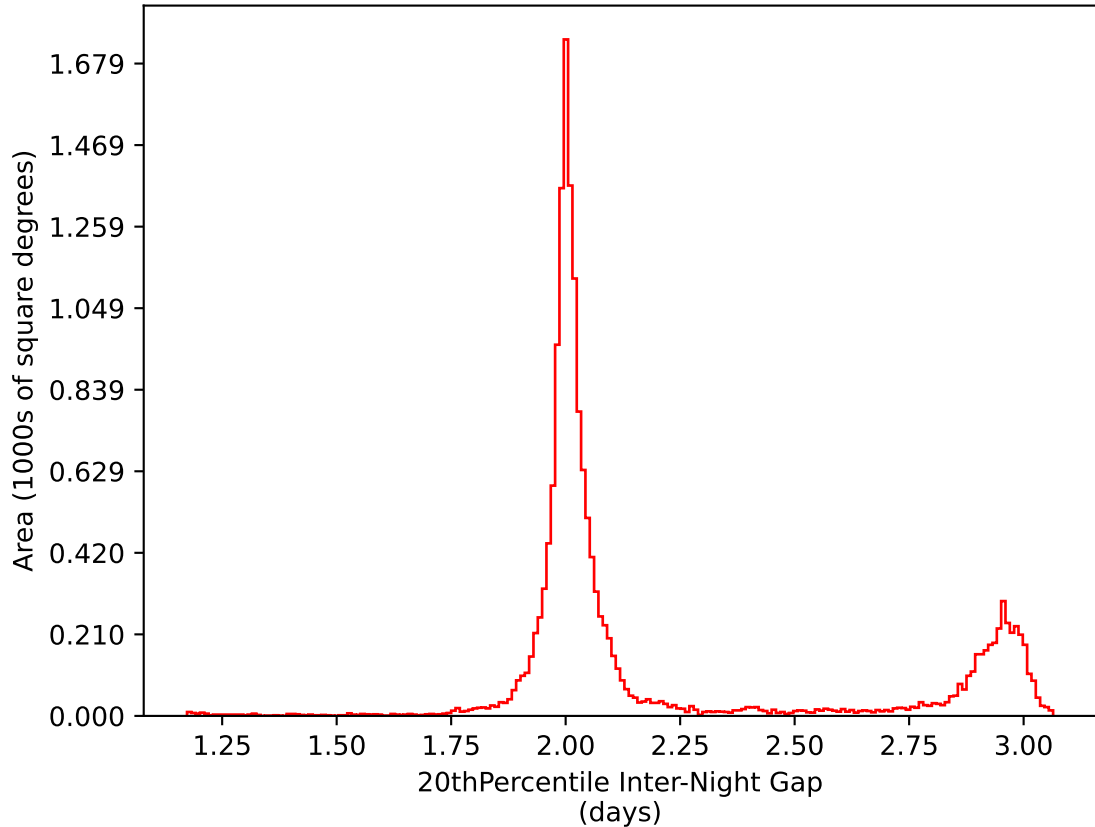
too_elab_r8_d3_giz_v3.4_10yrs WFD i band: 20thPercentile Inter-Night Gap
