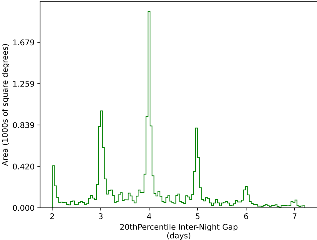
too_elab_r8_d3_giz_v3.4_10yrs WFD g band: 20thPercentile Inter-Night Gap
