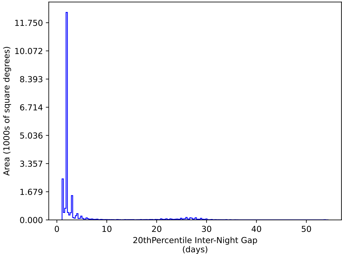
too_elab_r8_d3_giz_v3.4_10yrs All sky y band: 20thPercentile Inter-Night Gap
