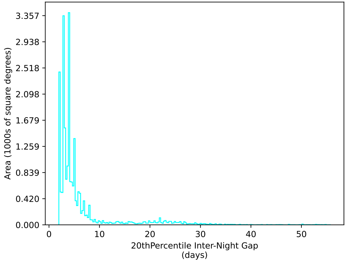
too_elab_r8_d3_giz_v3.4_10yrs All sky u band: 20thPercentile Inter-Night Gap
