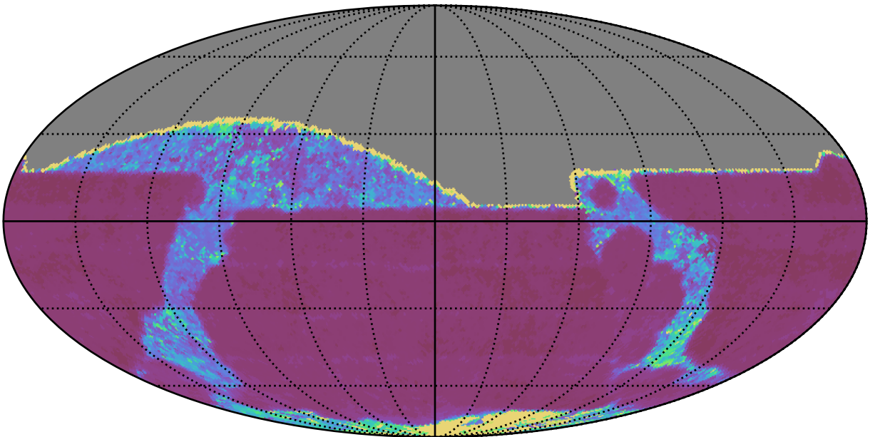
too_elab_r8_d3_giz_v3.4_10yrs All sky r band: 20thPercentile Inter-Night Gap
