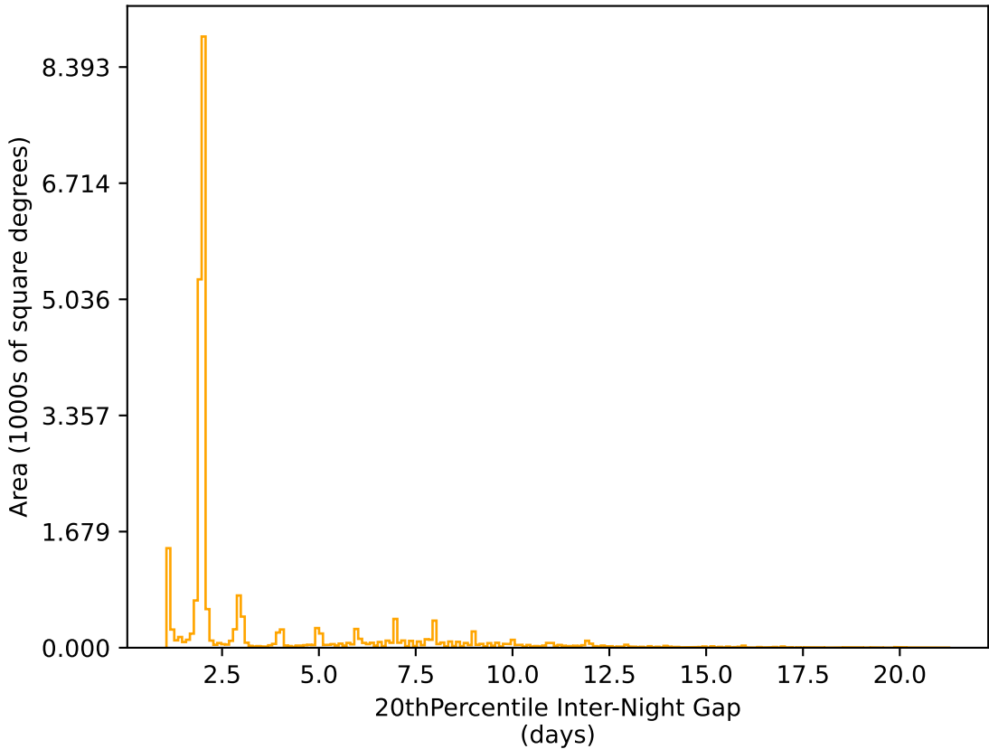
too_elab_r8_d3_giz_v3.4_10yrs All sky r band: 20thPercentile Inter-Night Gap
