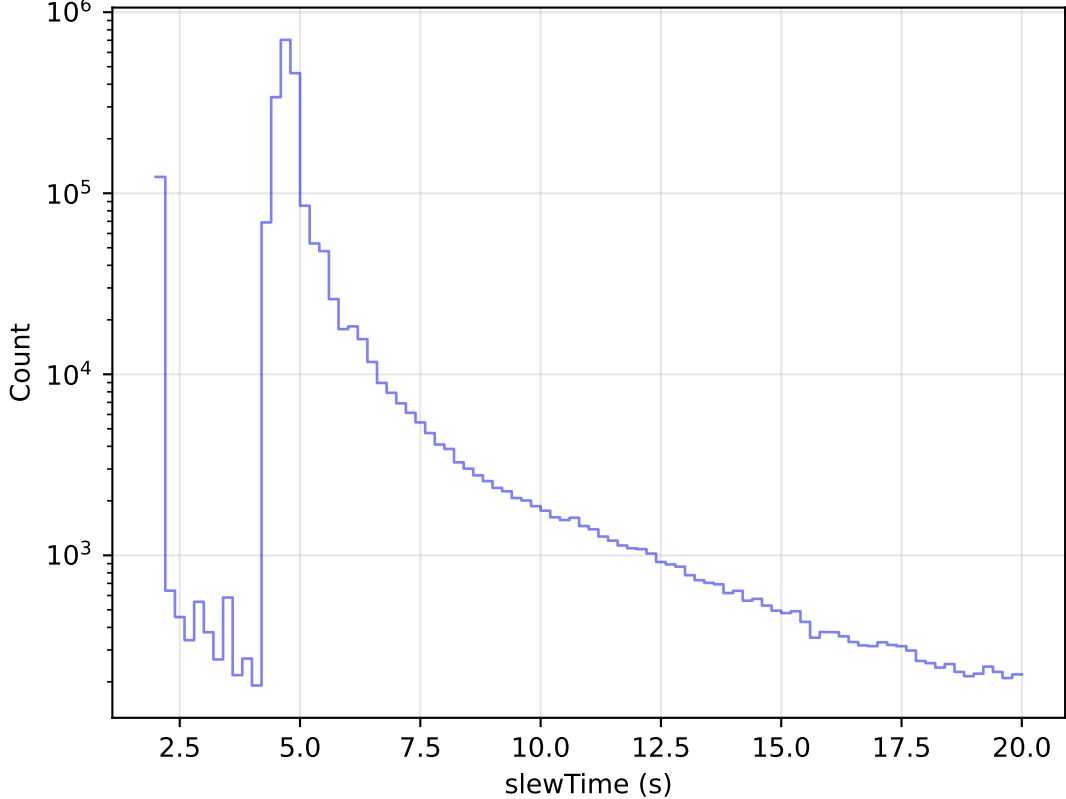
too_elab_r8_d3_giz_v3.4_10yrs All visits: Zoom Slew Time Histogram
