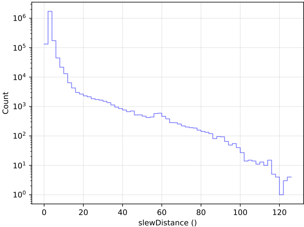
too_elab_r8_d3_giz_v3.4_10yrs All visits: Slew Distance Histogram
