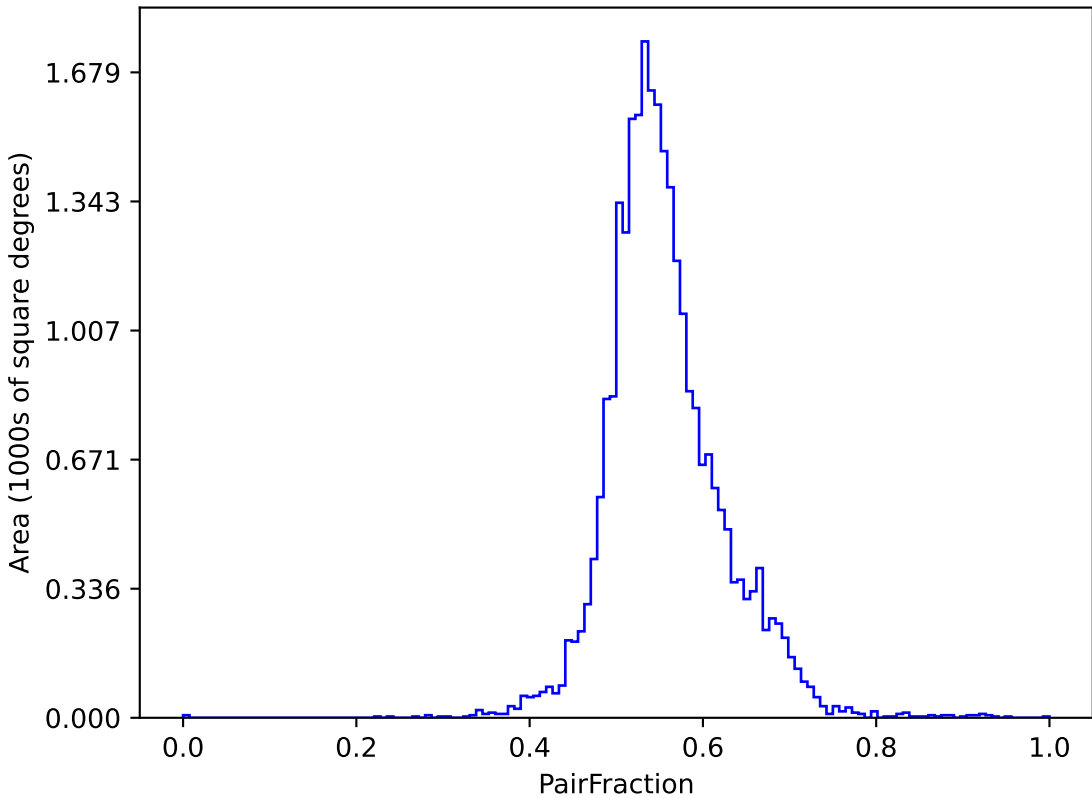
too_elab_r8_d3_giz_v3.4_10yrs (g or r or i): PairFraction
