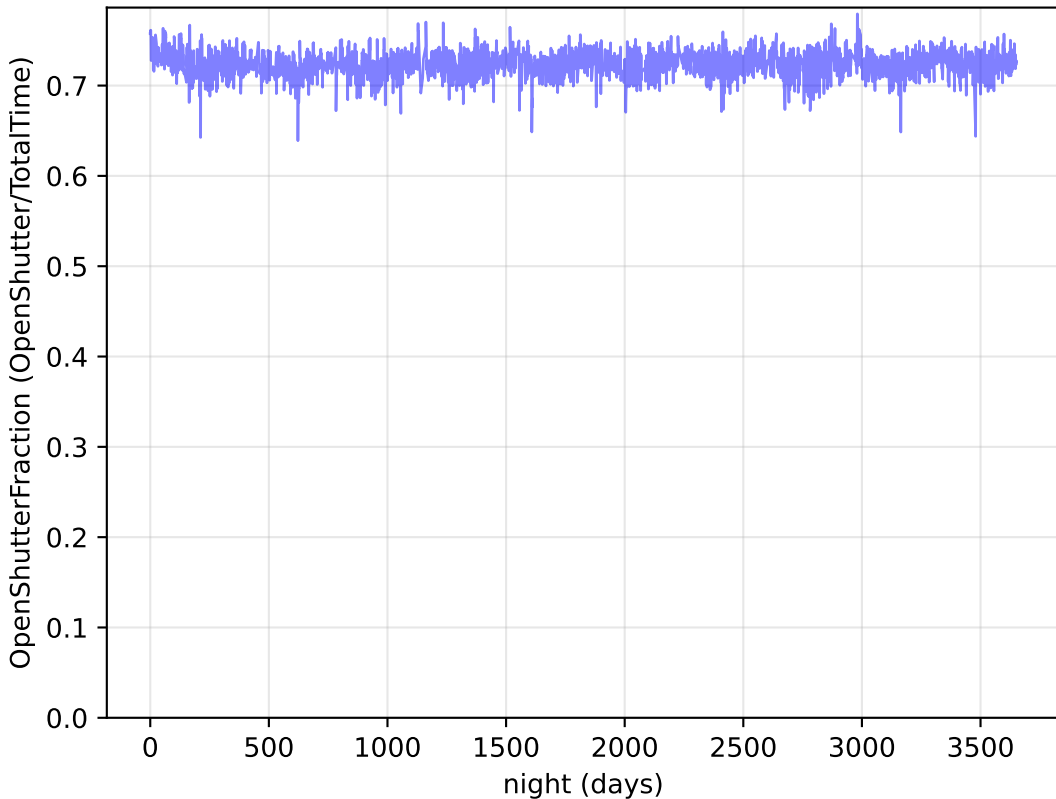
too_elab_r8_d3_giz_v3.4_10yrs : OpenShutterFraction
