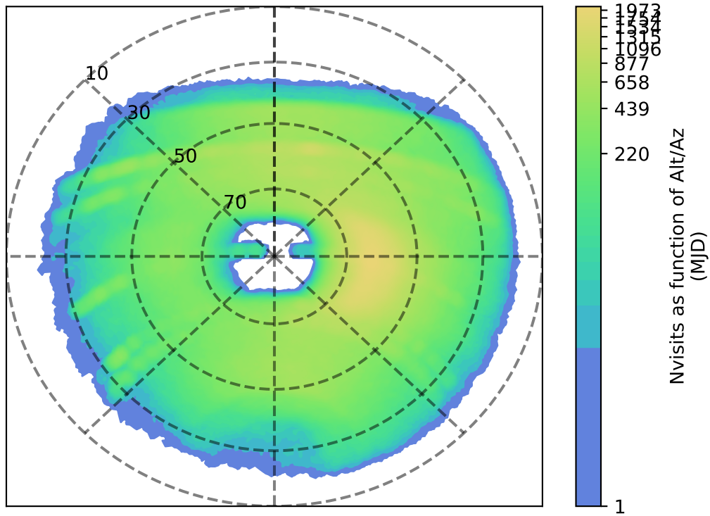
too_elab_r8_d3_giz_v3.4_10yrs y: Nvisits as function of Alt/Az
