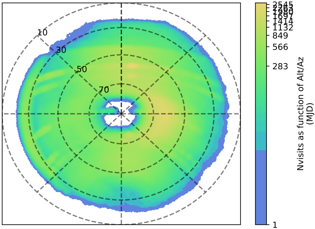
too_elab_r8_d3_giz_v3.4_10yrs r: Nvisits as function of Alt/Az
