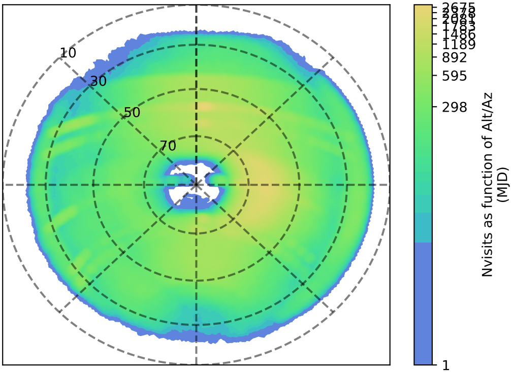
too_elab_r8_d3_giz_v3.4_10yrs i: Nvisits as function of Alt/Az
