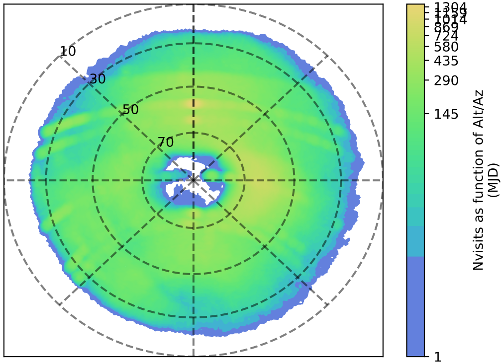
too_elab_r8_d3_giz_v3.4_10yrs g: Nvisits as function of Alt/Az
