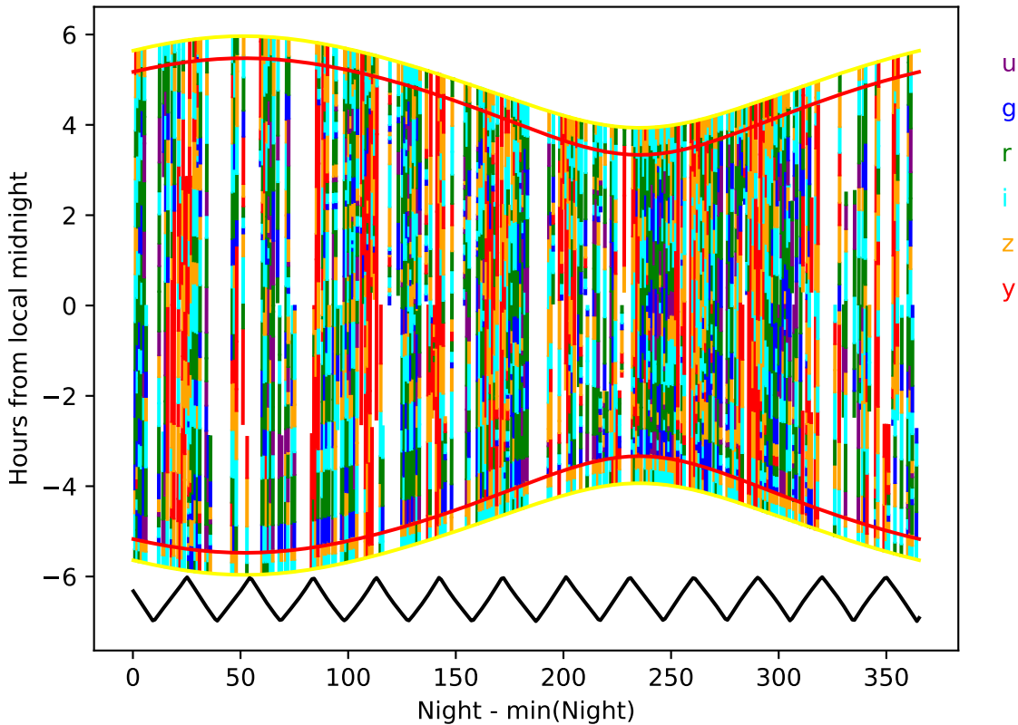
too_elab_r8_d3_giz_v3.4_10yrs year 7-8: Hourglass
