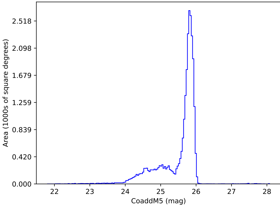
too_elab_r8_d3_giz_v3.4_10yrs z: CoaddM5
