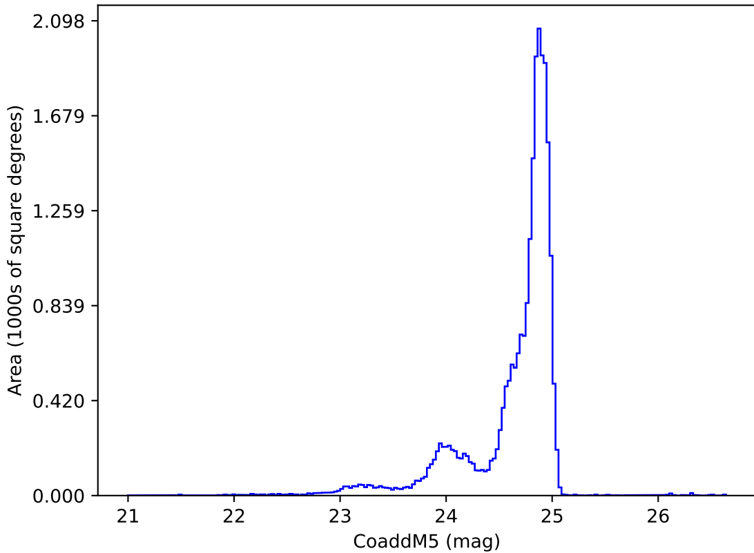
too_elab_r8_d3_giz_v3.4_10yrs y: CoaddM5
