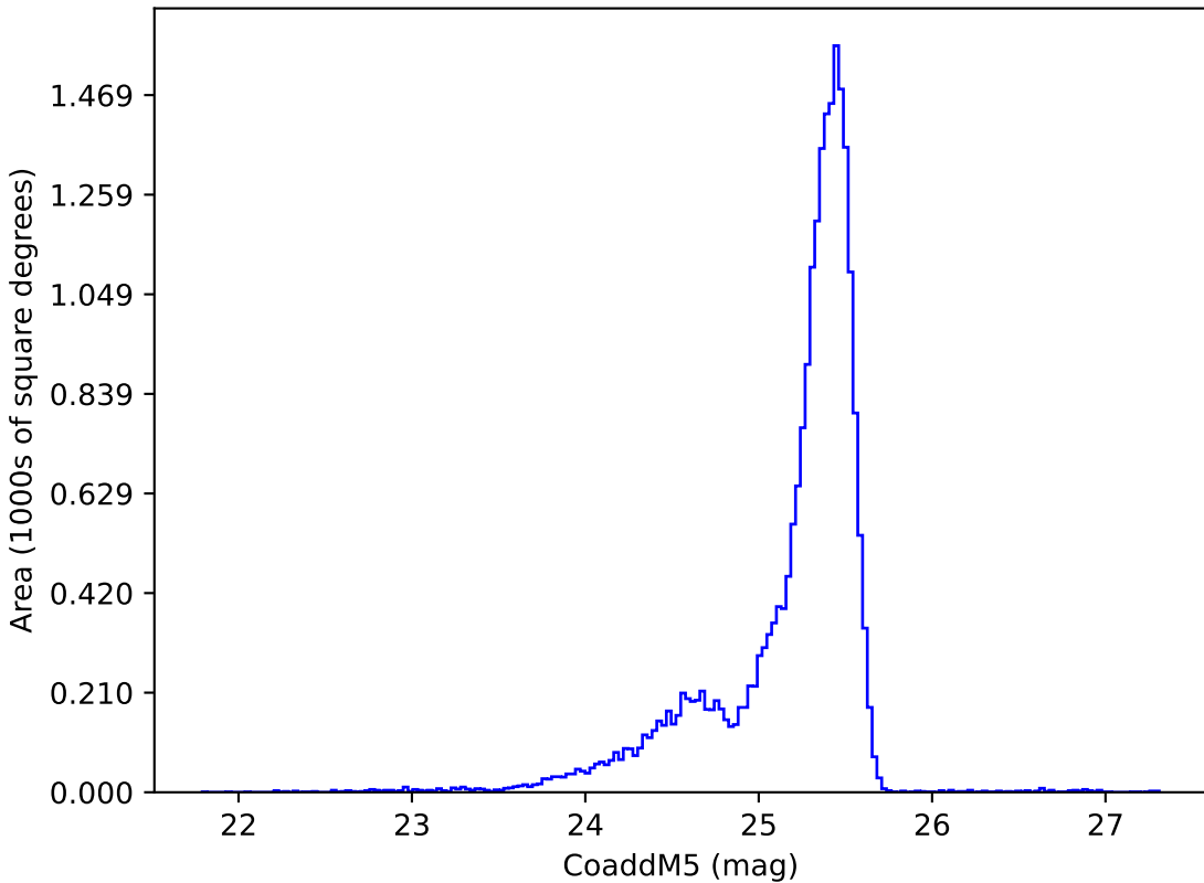
too_elab_r8_d3_giz_v3.4_10yrs u: CoaddM5
