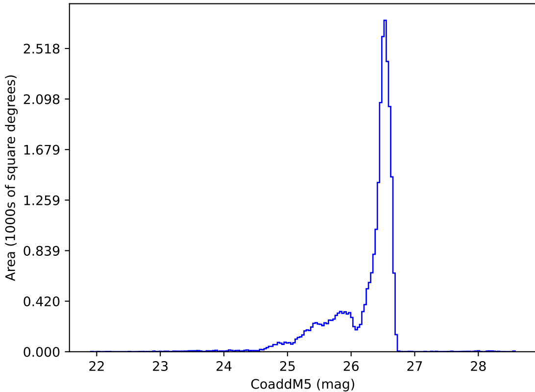
too_elab_r8_d3_giz_v3.4_10yrs i: CoaddM5
