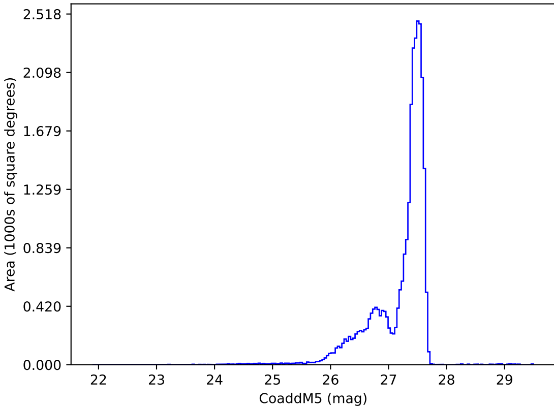
too_elab_r8_d3_giz_v3.4_10yrs : CoaddM5
