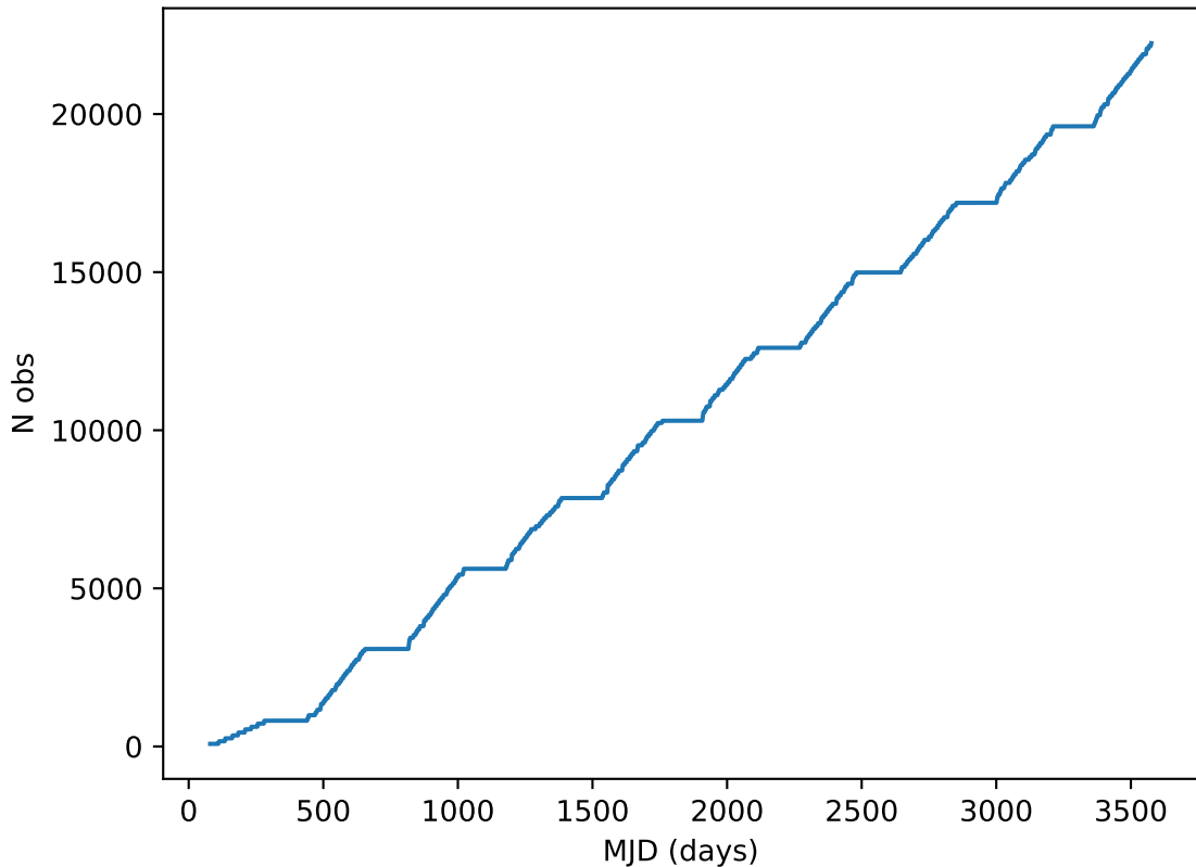
too_elab_r8_d3_giz_v3.4_10yrs all bands: DD:XMM_LSS Cumulative NVisits
