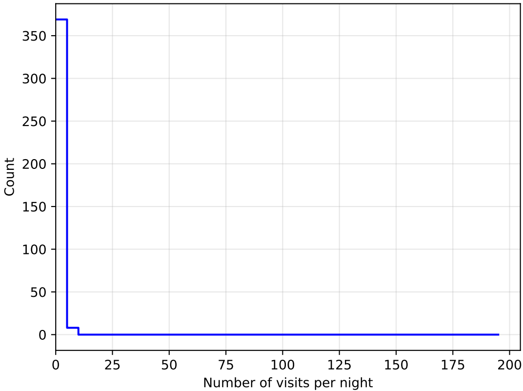
too_elab_r8_d3_giz_v3.4_10yrs all bands: DD:WFD NVisitsPerNight
