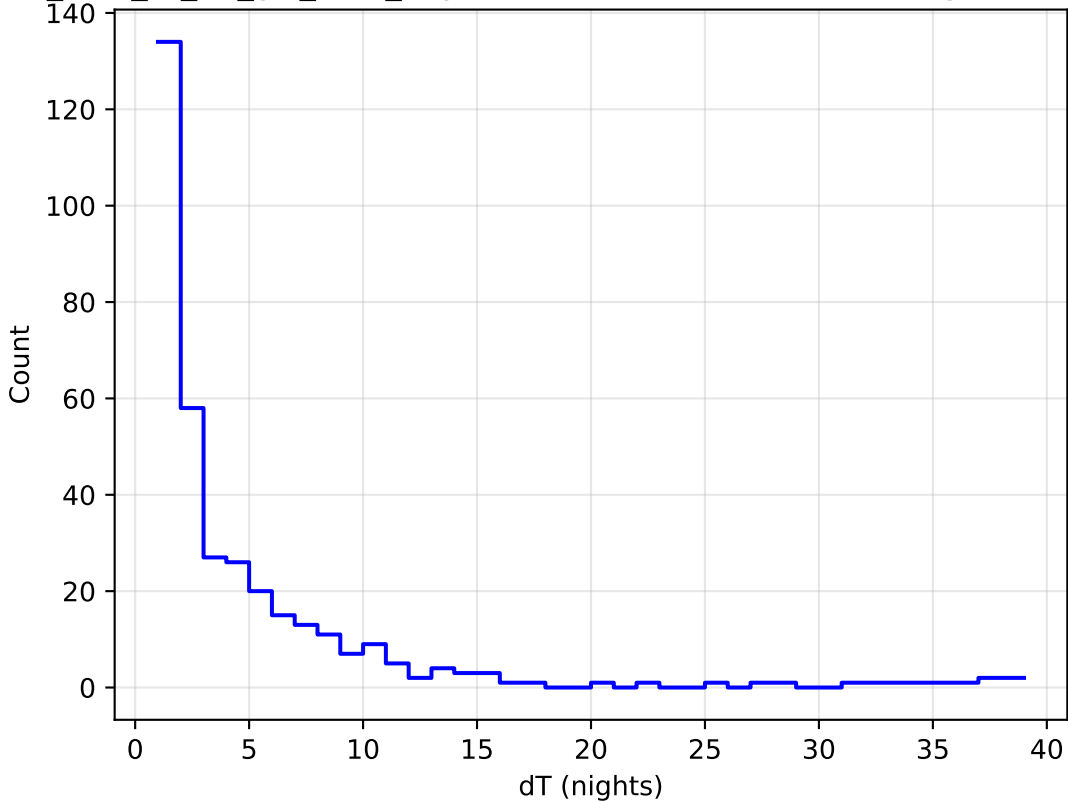
too_elab_r8_d3_giz_v3.4_10yrs all bands: DD:WFD Delta Nights Histogram
