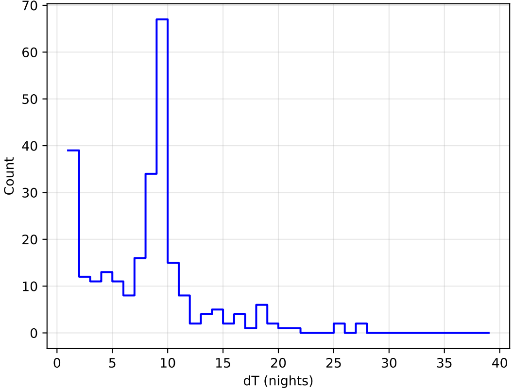
too_elab_r8_d3_giz_v3.4_10yrs all bands: DD:ELAISS1 Delta Nights Histogram
