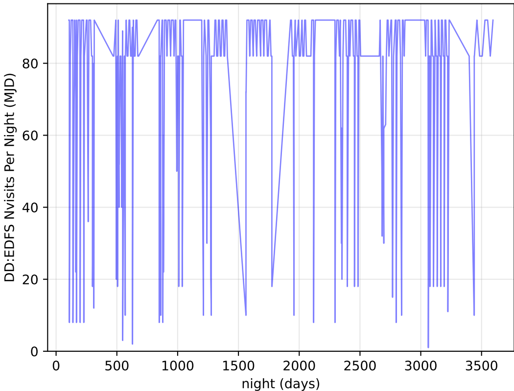
too_elab_r8_d3_giz_v3.4_10yrs all bands: DD:EDFS Nvisits Per Night
