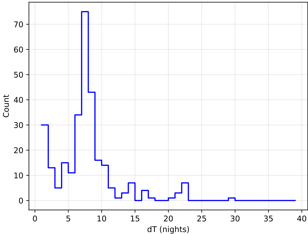
too_elab_r8_d3_giz_v3.4_10yrs all bands: DD:EDFS Delta Nights Histogram
