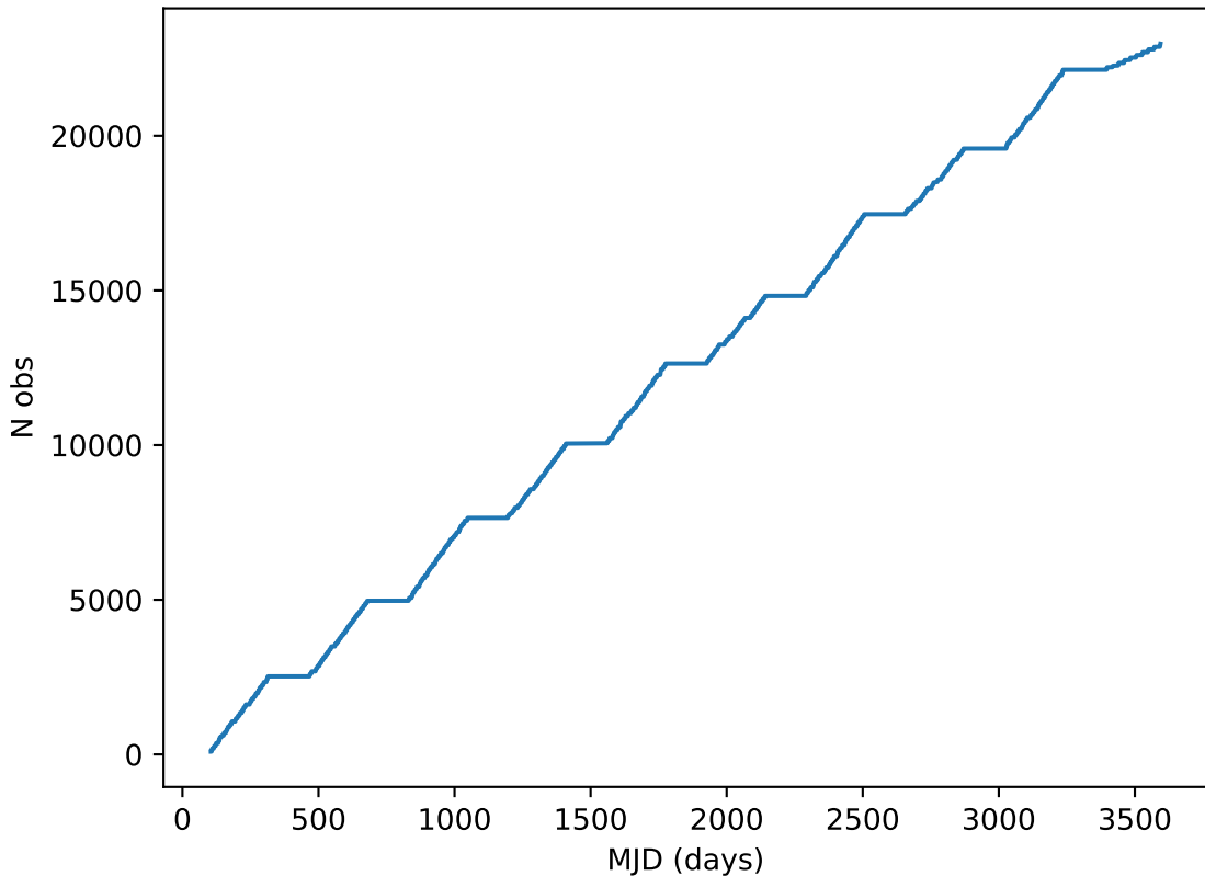
too_elab_r8_d3_giz_v3.4_10yrs all bands: DD:EDFS Cumulative NVisits
