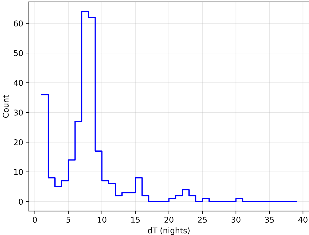
too_elab_r8_d3_giz_v3.4_10yrs all bands: DD:ECDFS Delta Nights Histogram
