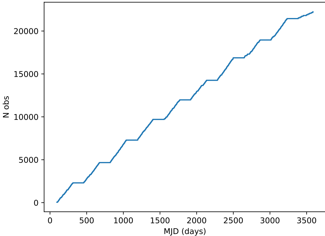
too_elab_r8_d3_giz_v3.4_10yrs all bands: DD:ECDFS Cumulative NVisits
