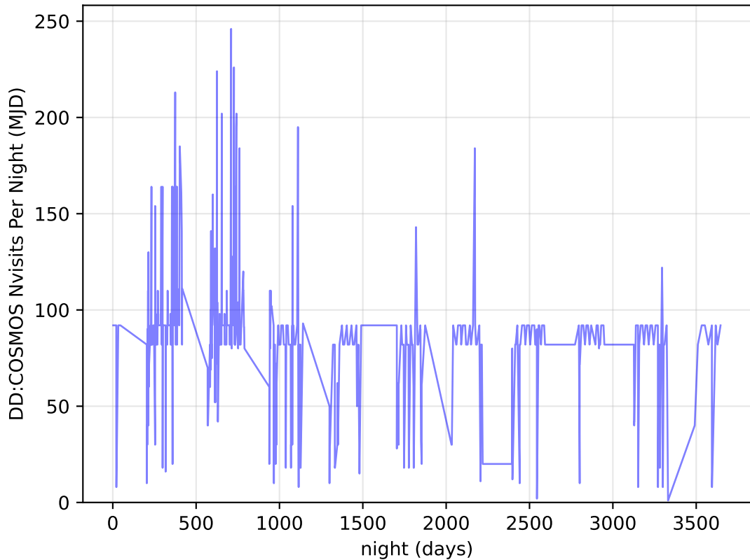
too_elab_r8_d3_giz_v3.4_10yrs all bands: DD: COSMOS Nvisits Per Night
