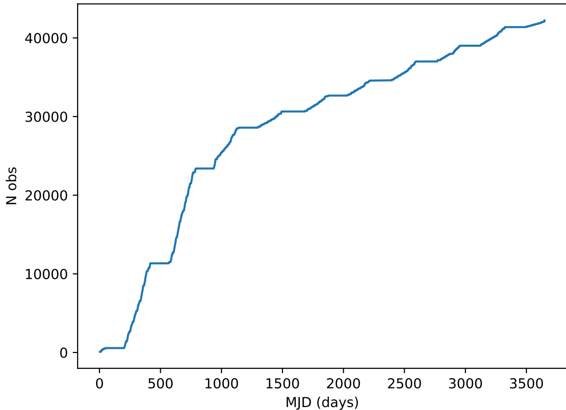
too_elab_r8_d3_giz_v3.4_10yrs all bands: DD: COSMOS Cumulative NVisits
