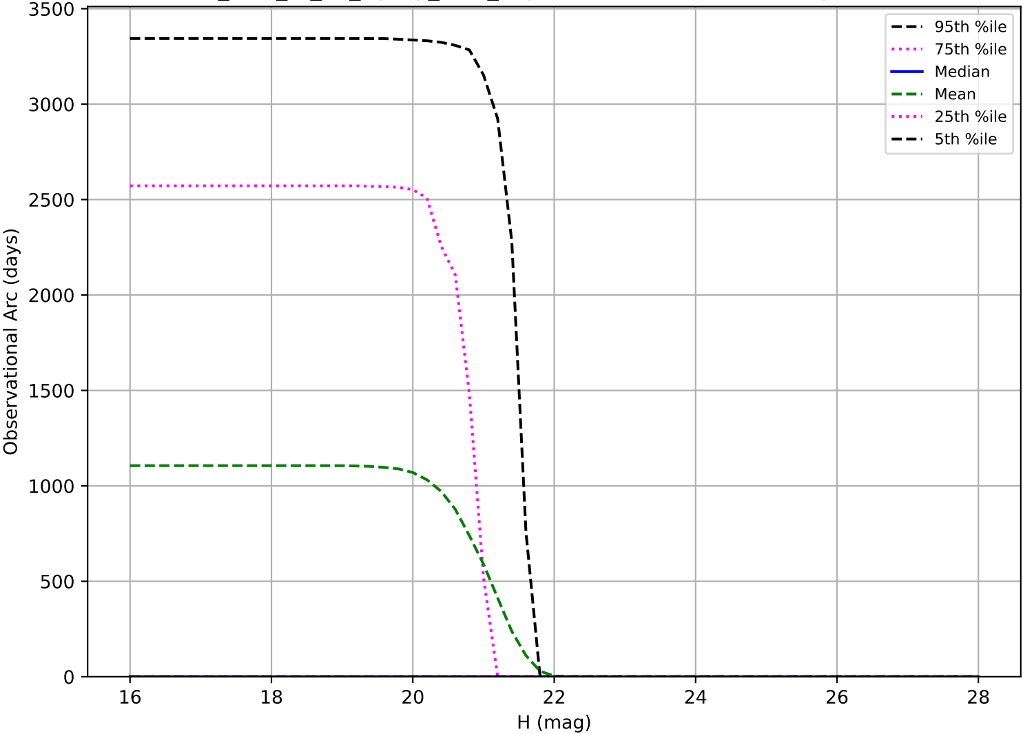
too_elab_r8_d2_ugrizy_v3.4_10yrs: Observational Arc Length Vatira
