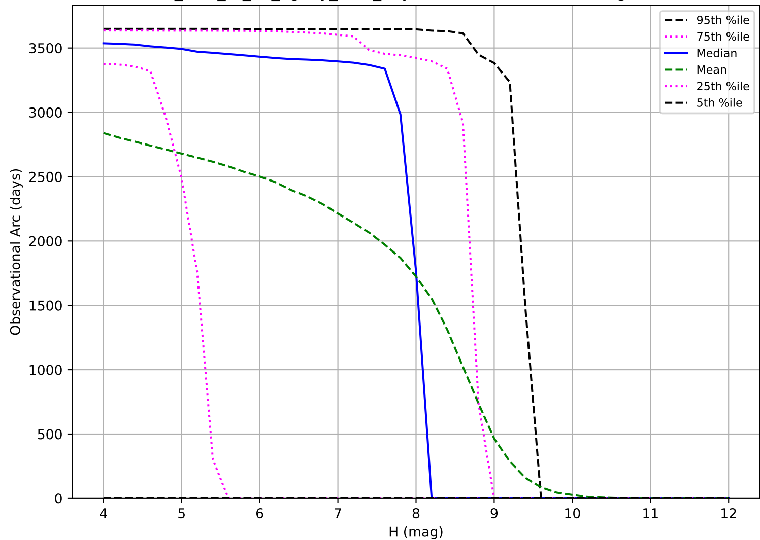
too_elab_r8_d2_ugrizy_v3.4_10yrs: Observational Arc Length TNO
