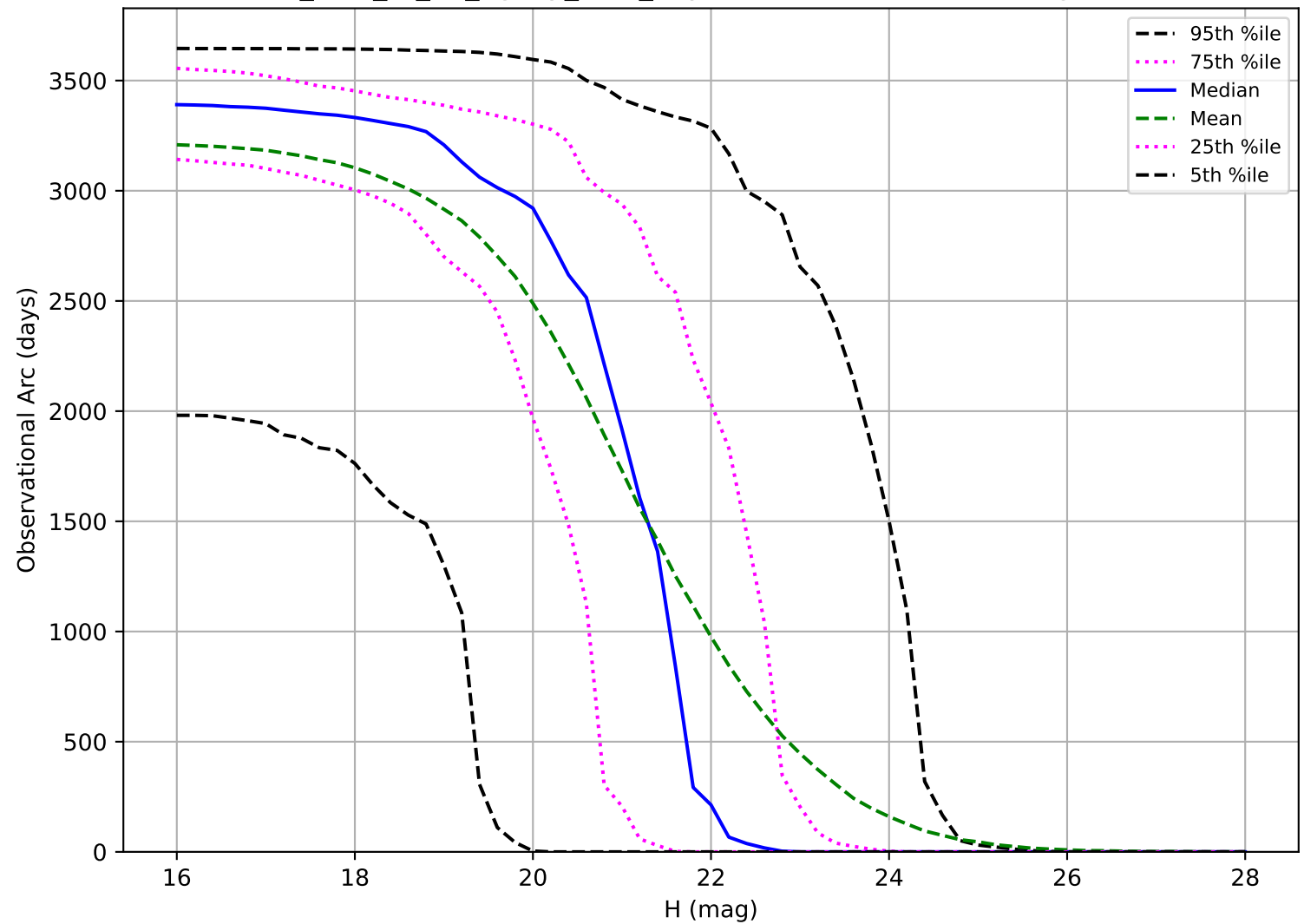
too_elab_r8_d2_ugrizy_v3.4_10yrs: Observational Arc Length PHA
