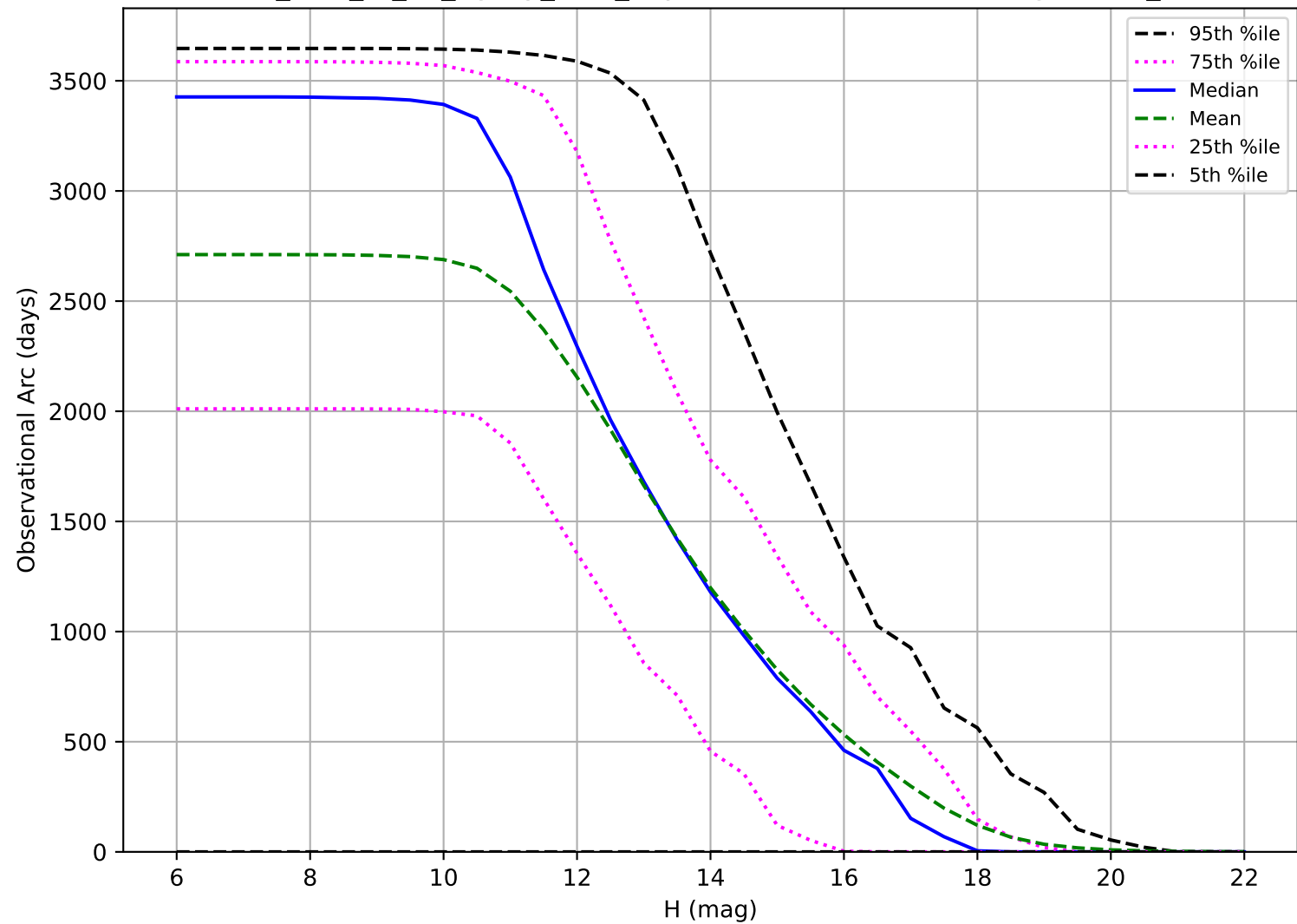
too_elab_r8_d2_ugrizy_v3.4_10yrs: Observational Arc Length OCC_r5
