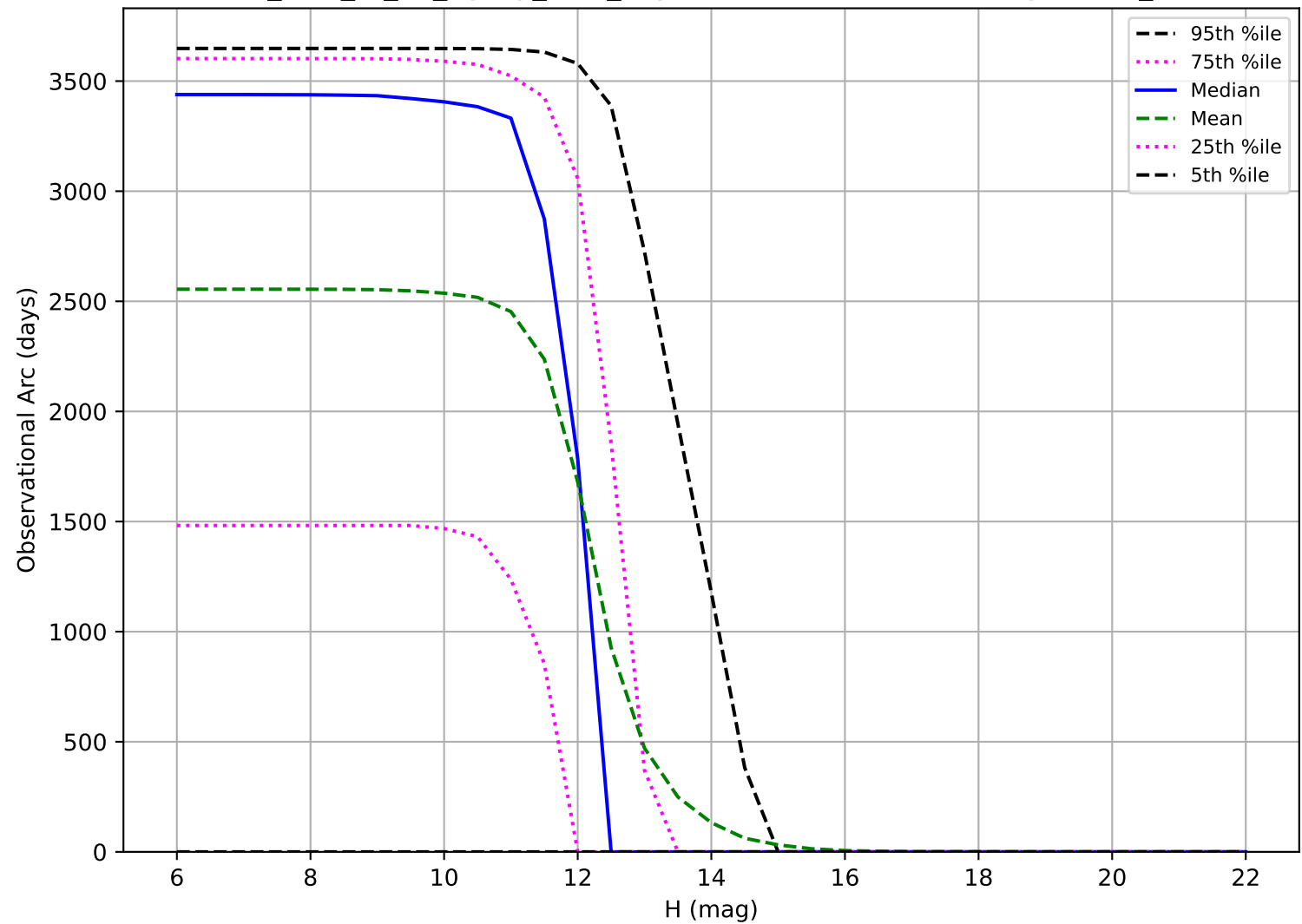
too_elab_r8_d2_ugrizy_v3.4_10yrs: Observational Arc Length OCC_r20
