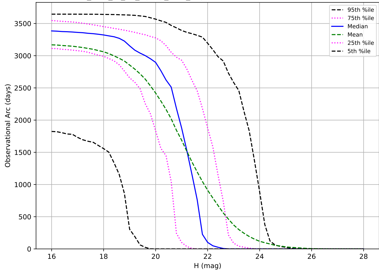
too_elab_r8_d2_ugrizy_v3.4_10yrs: Observational Arc Length NEO
