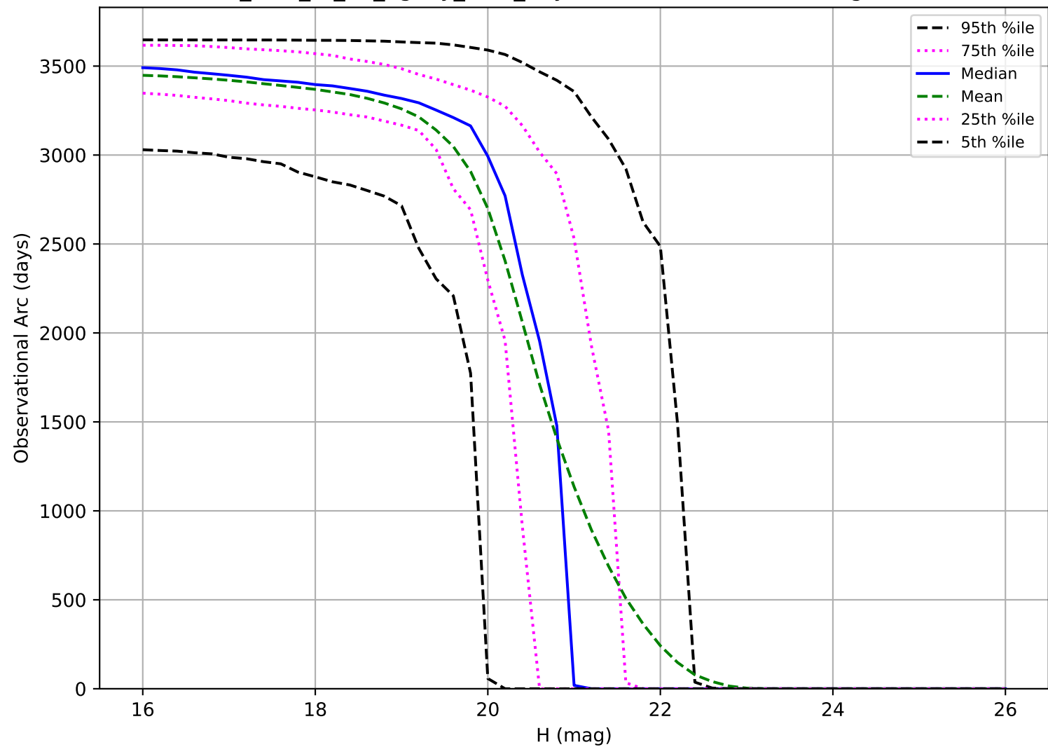
too_elab_r8_d2_ugrizy_v3.4_10yrs: Observational Arc Length MBA
