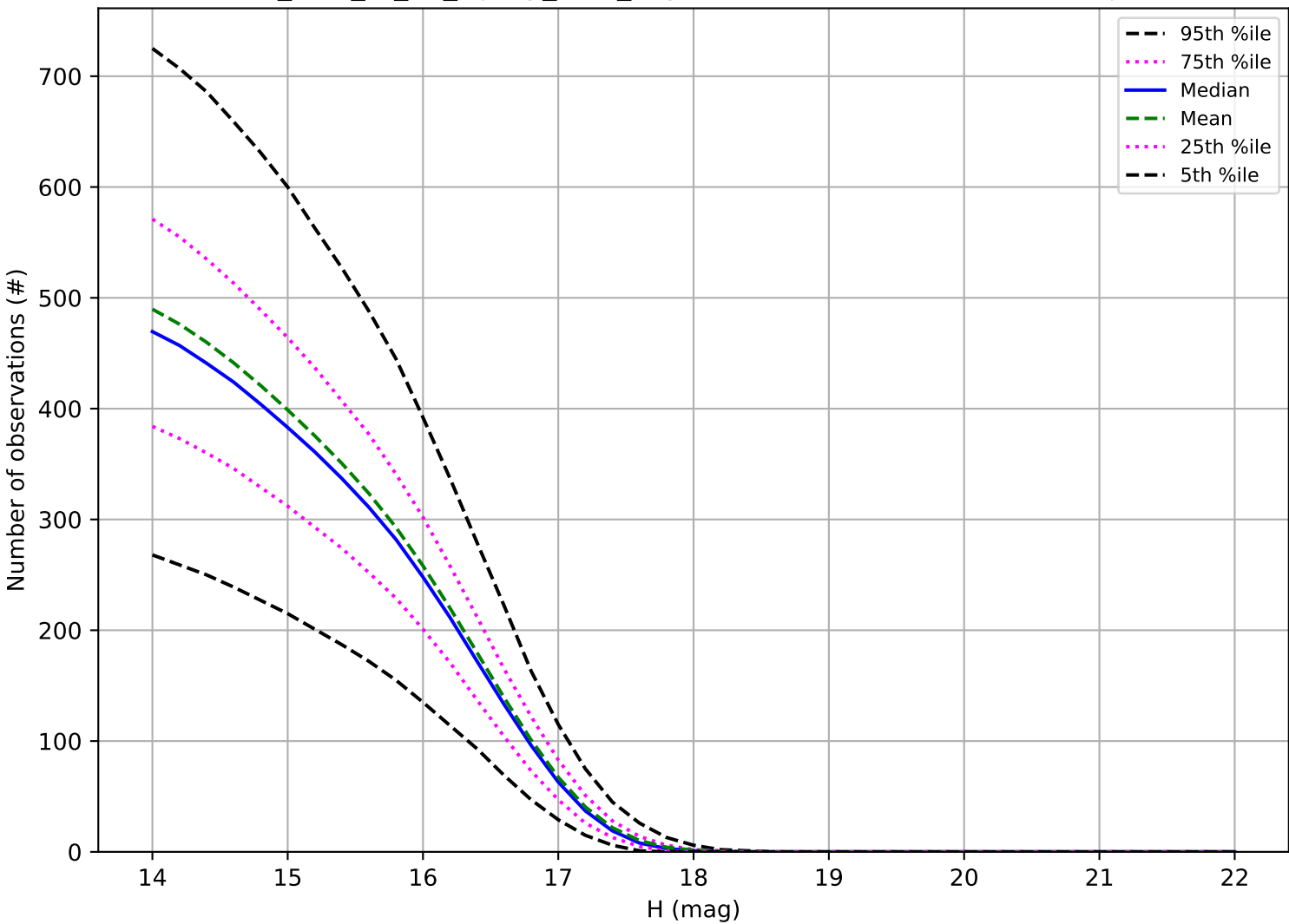
too_elab_r8_d2_ugrizy_v3.4_10yrs: Number of observations Trojan
